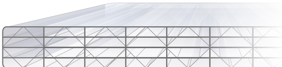
5-Wall X-structure
